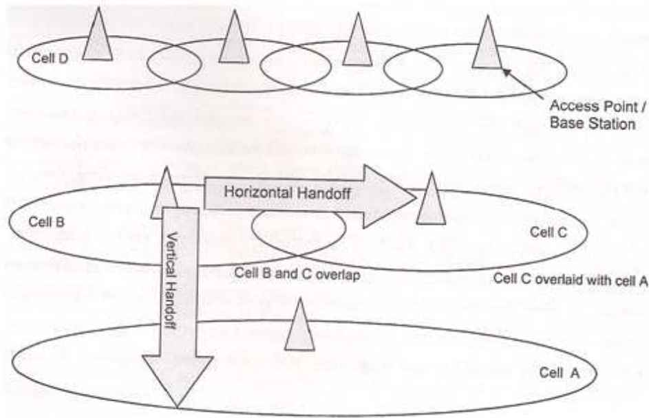
Figure 2. Horizontal and vertical handoffs.
